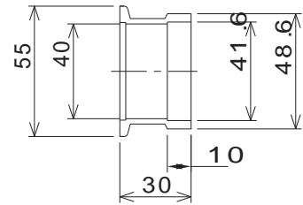
CCF-40
