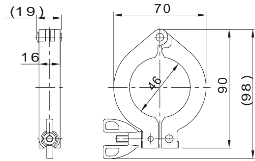
CCR-40
