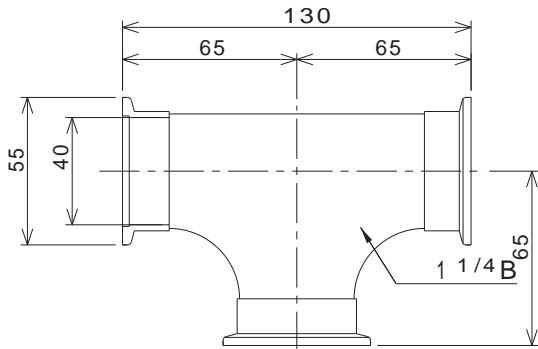
TC-40
